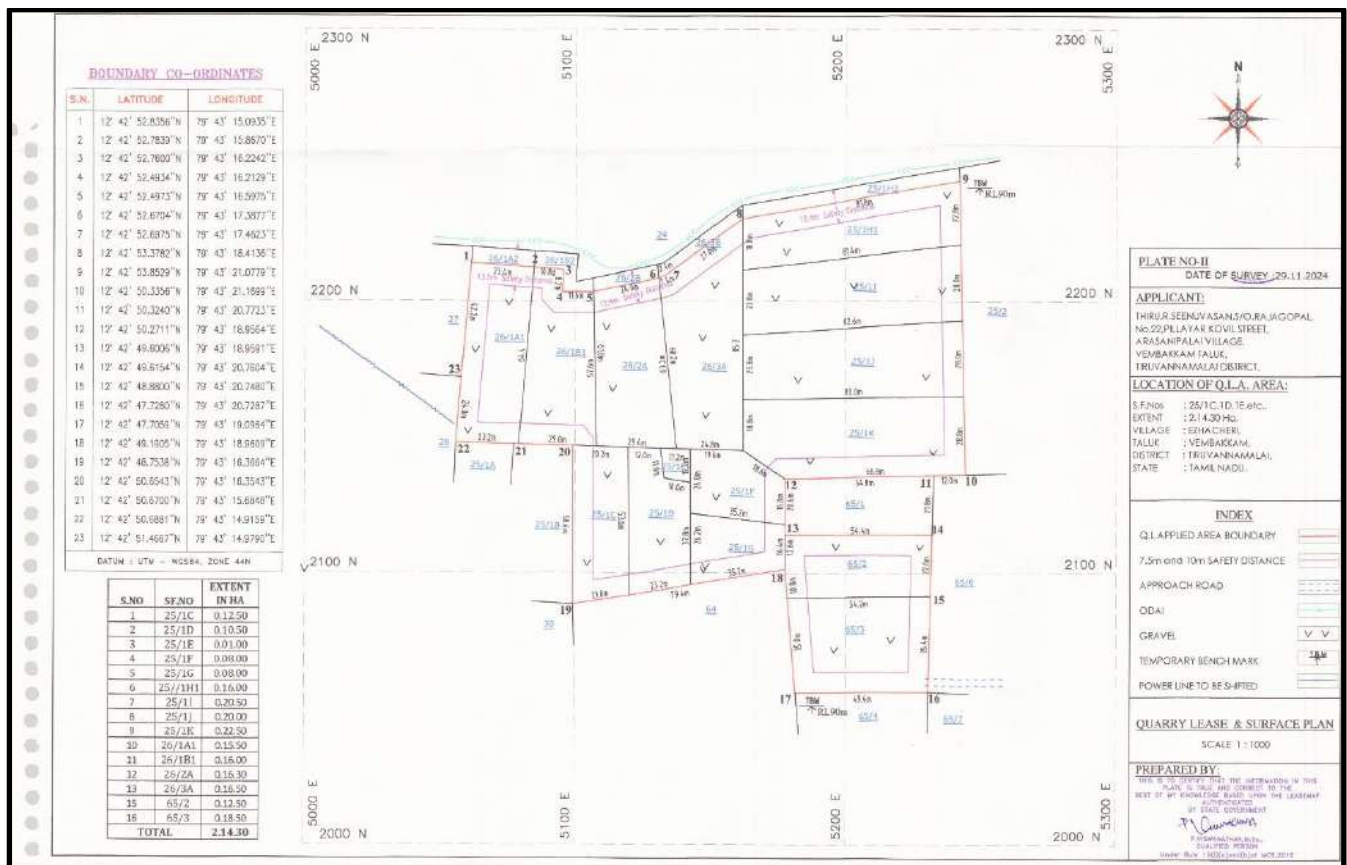
FIGURE 3: QUARRY LEASE PLAN / SURFACE PLAN
