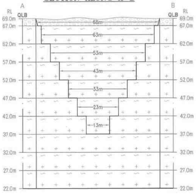
SECTION ALONG A-B
