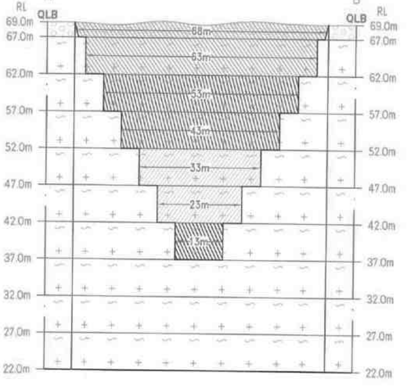
SECTION ALONG A-B
