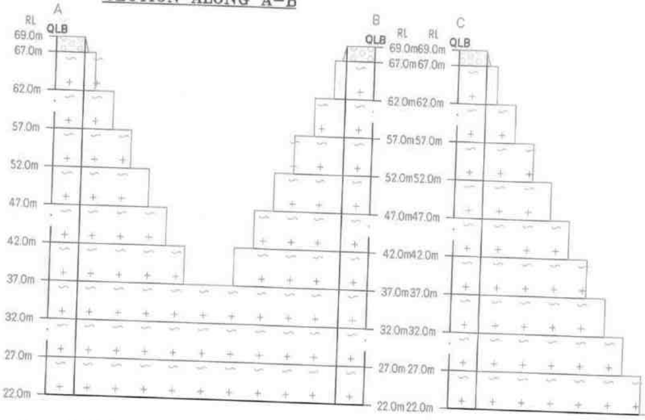
SECTION ALONG A-B
