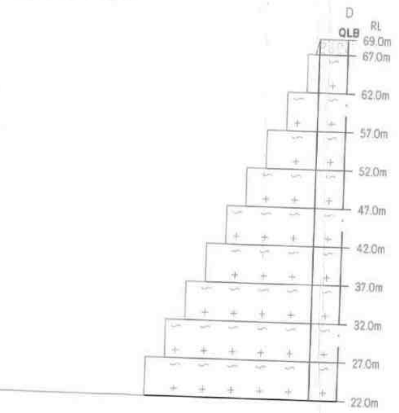
SECTION ALONG C-D
