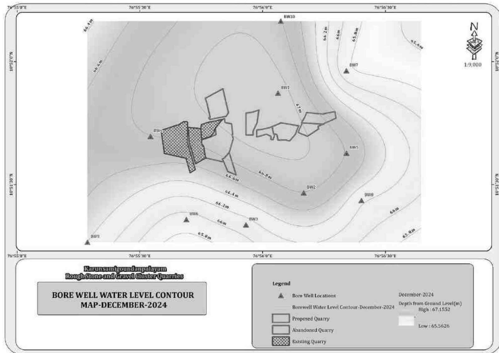
FIGURE 3.11: BOREWELL CONTOUR MAP – DECEMBER 2024
