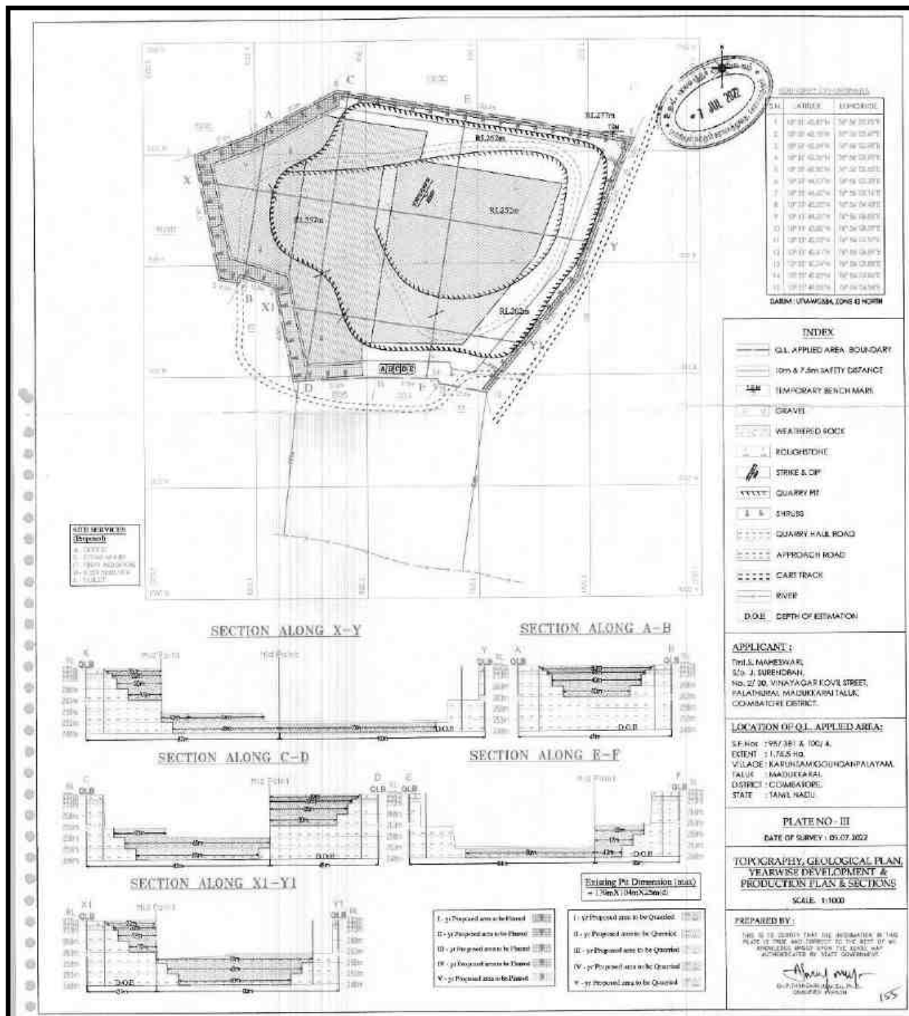
FIGURE 2.15: TOPOGRAPHY, GEOLOGICAL, YEAR-WISE DEVELOPMENT PRODUCTION PLAN AND SECTIONS – P1
