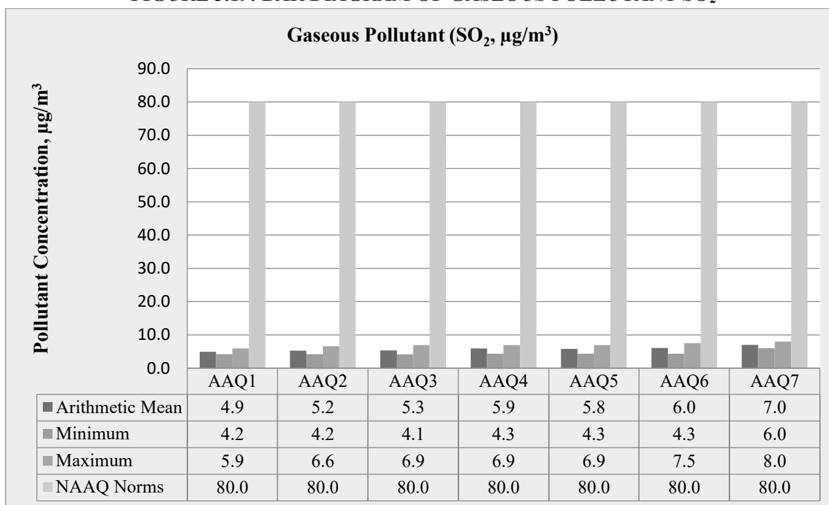
FIGURE 3.19: BAR DIAGRAM OF GASEOUS POLLUTANT SO 2
