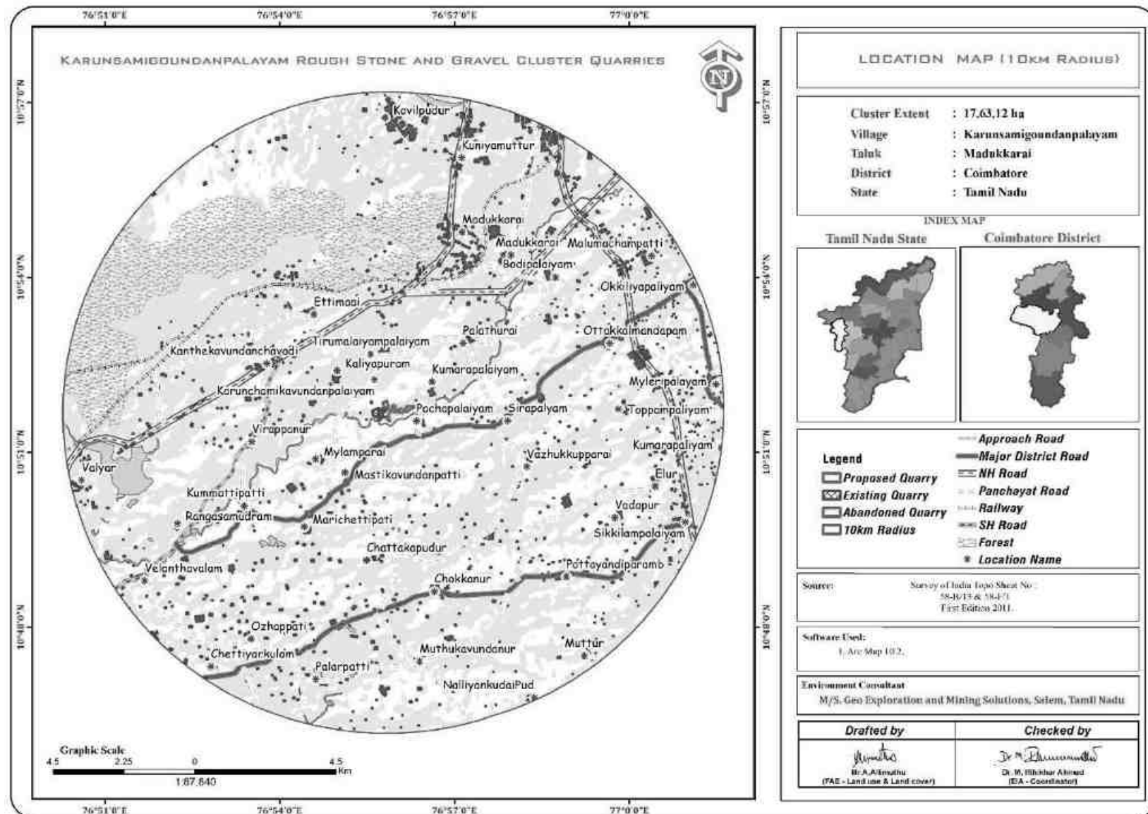
FIGURE 2.10: IMAGE SHOWING SURFACE FEATURES AROUND 10 KM RADIUS
