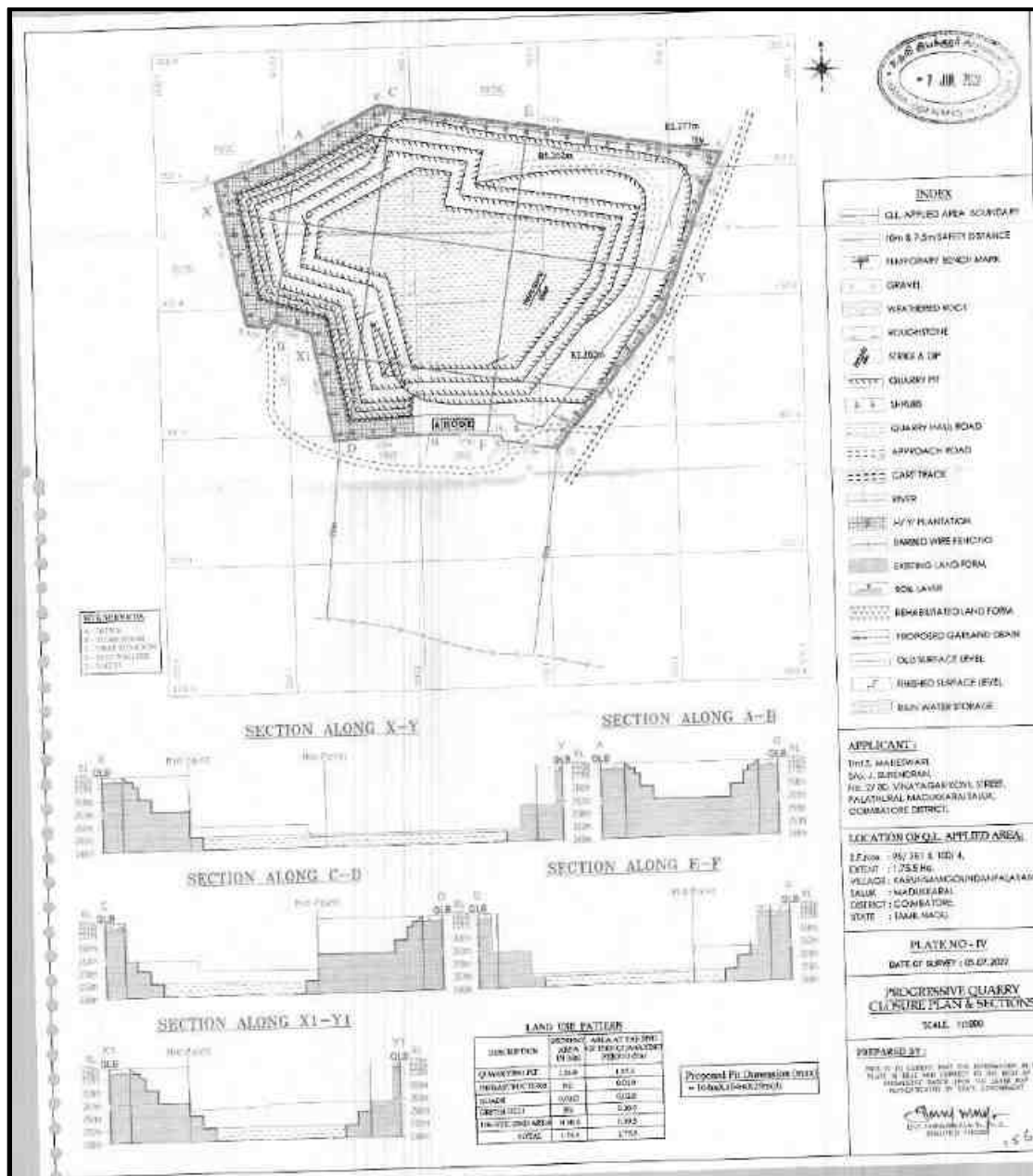
FIGURE 2.17: CLOSURE PLAN AND SECTIONS- P1
