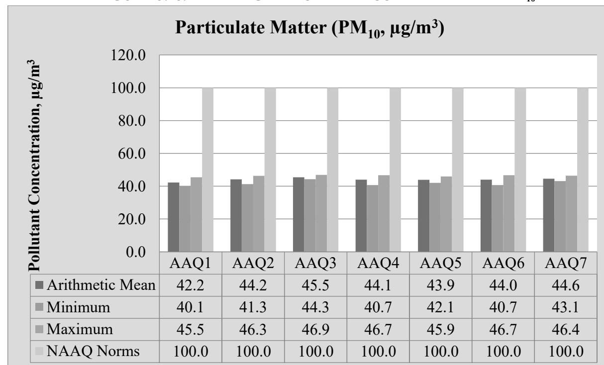
FIGURE 3.18: BAR DIAGRAM OF PARTICULATE MATTER PM 10
