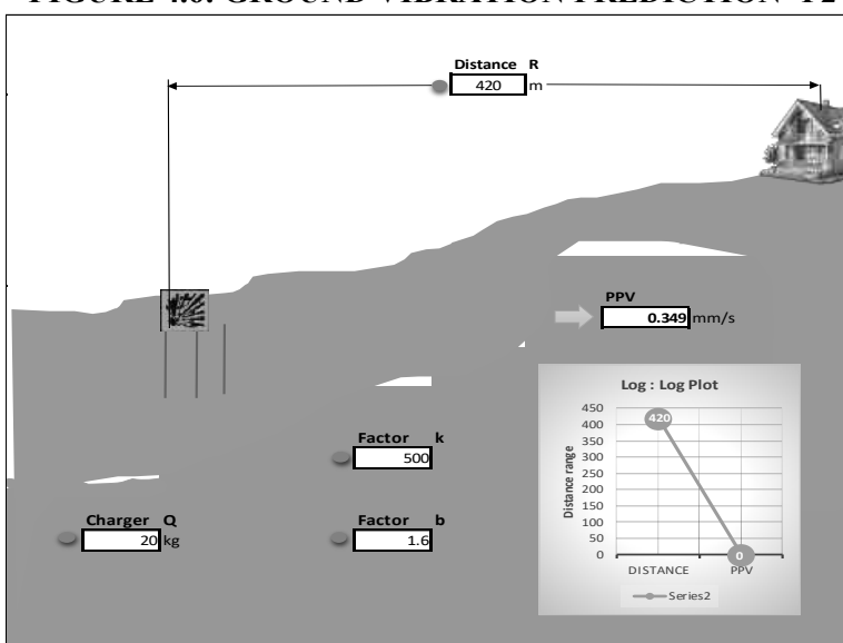
FIGURE 4.6: GROUND VIBRATION PREDICTION- P2
