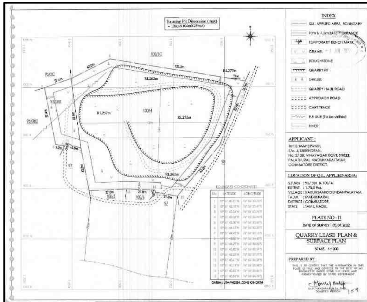
FIGURE 2.7: QUARRY LEASE PLAN / SURFACE PLAN- P1
