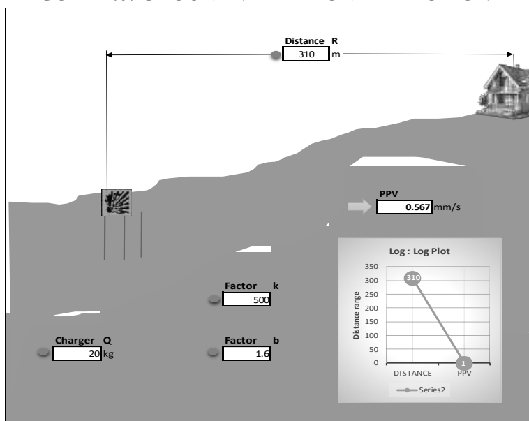
FIGURE 4.6: GROUND VIBRATION PREDICTION- P1
