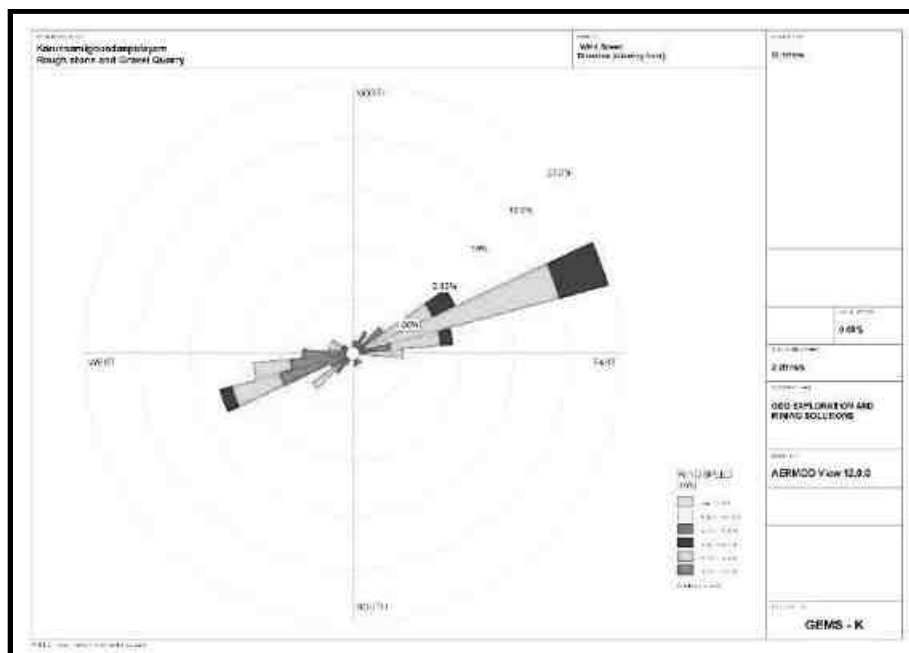
FIGURE 3.14: WINDROSE DIAGRAM
