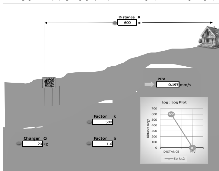
FIGURE 4.7: GROUND VIBRATION PREDICTION
