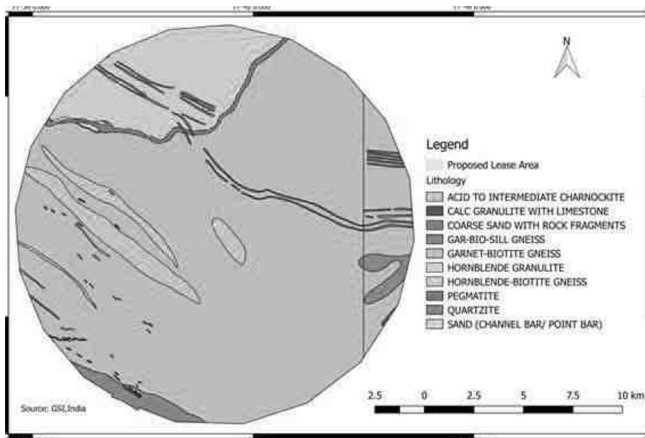
FIGURE 3.16 - LITHOLOGY BUFFER ZONE MAP
