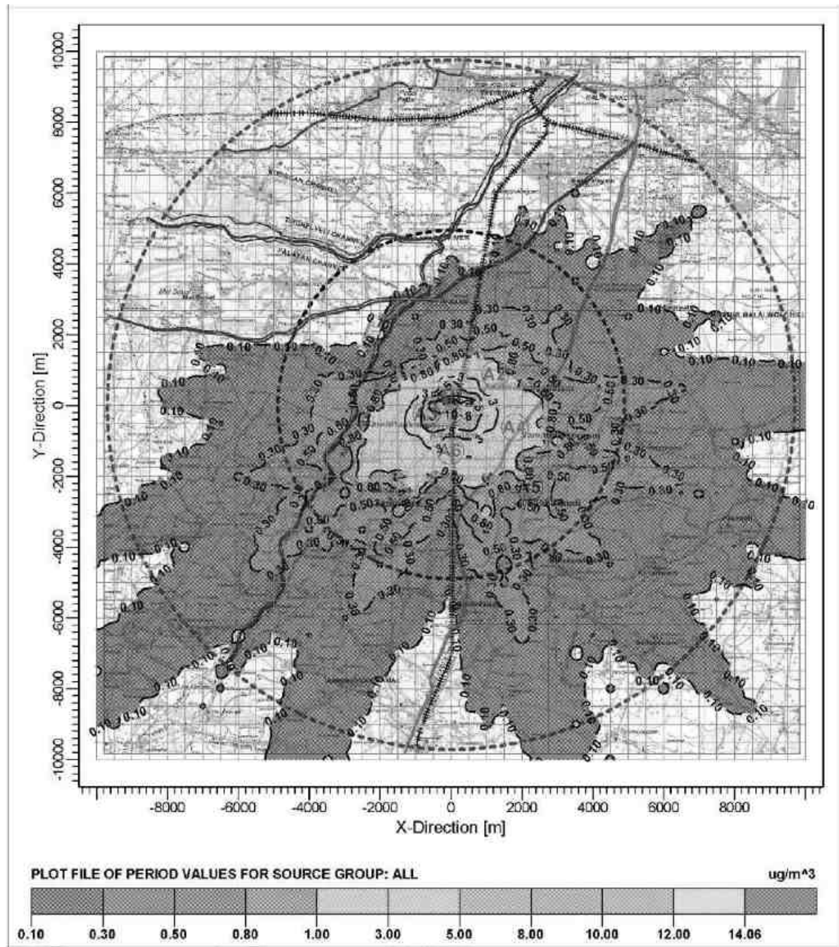
FIGURE 7.2 – CUMULATIVE ISOPLETH OF GLC PREDICTION FOR PM 10
