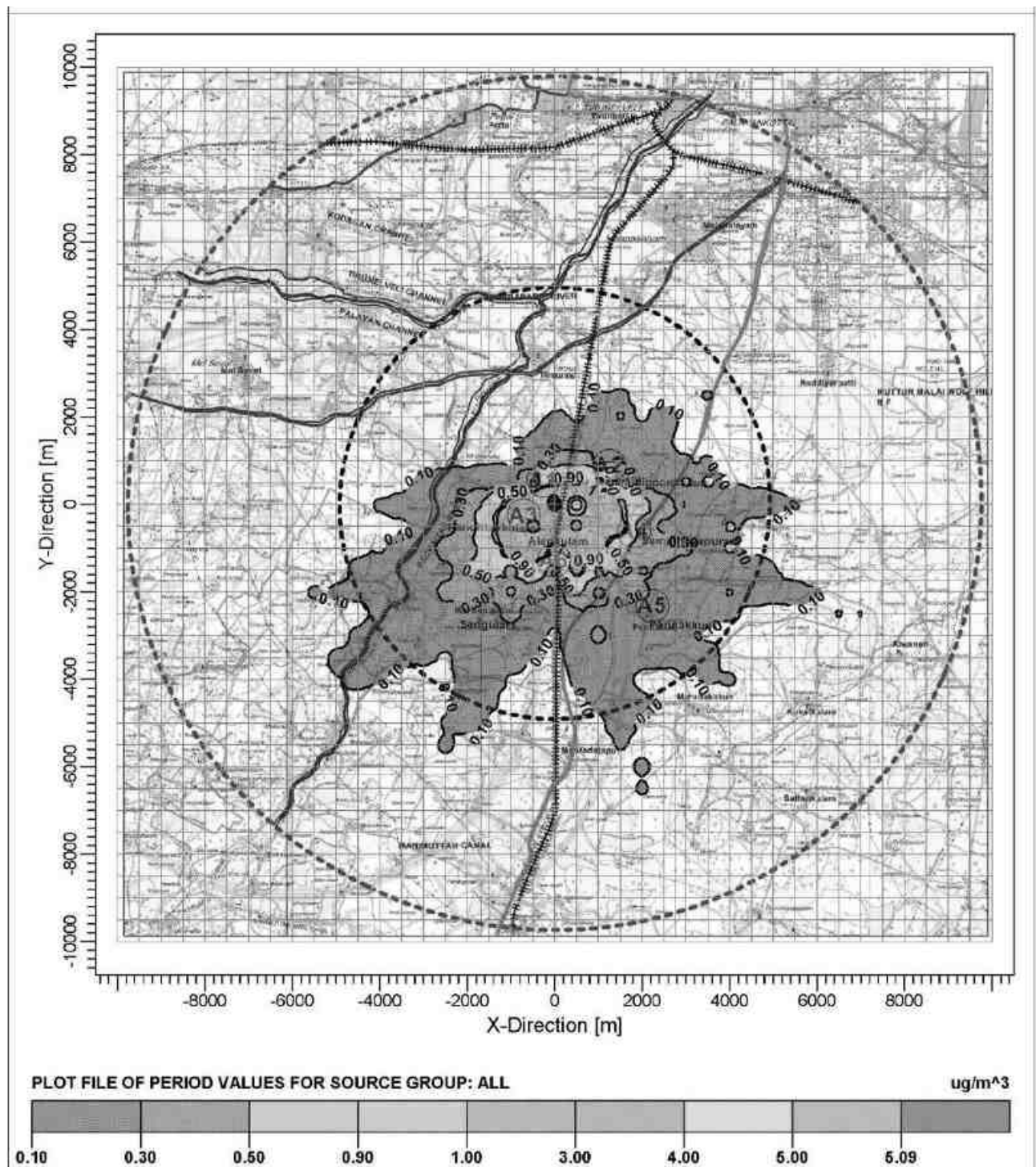
FIGURE 4.2 - ISOPLETH OF GLC PREDICTION FOR PM 10
