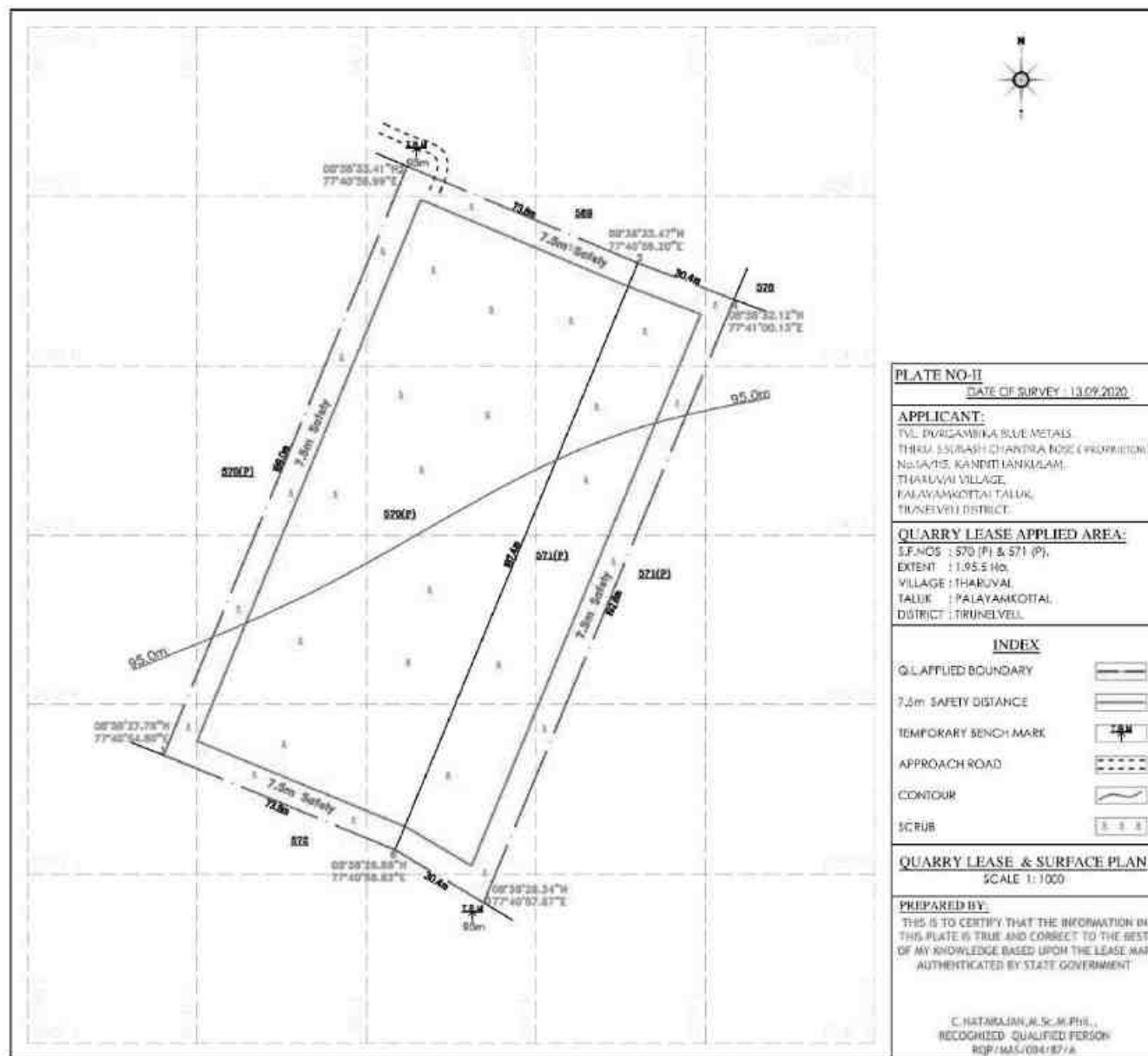
FIGURE 2.3 - SURFACE PLAN OF THE PROJECT AREA
