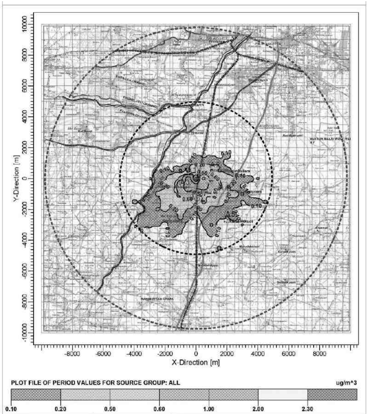
FIGURE 4.3 - ISOPLETH OF GLC PREDICTION FOR PM 2.5
